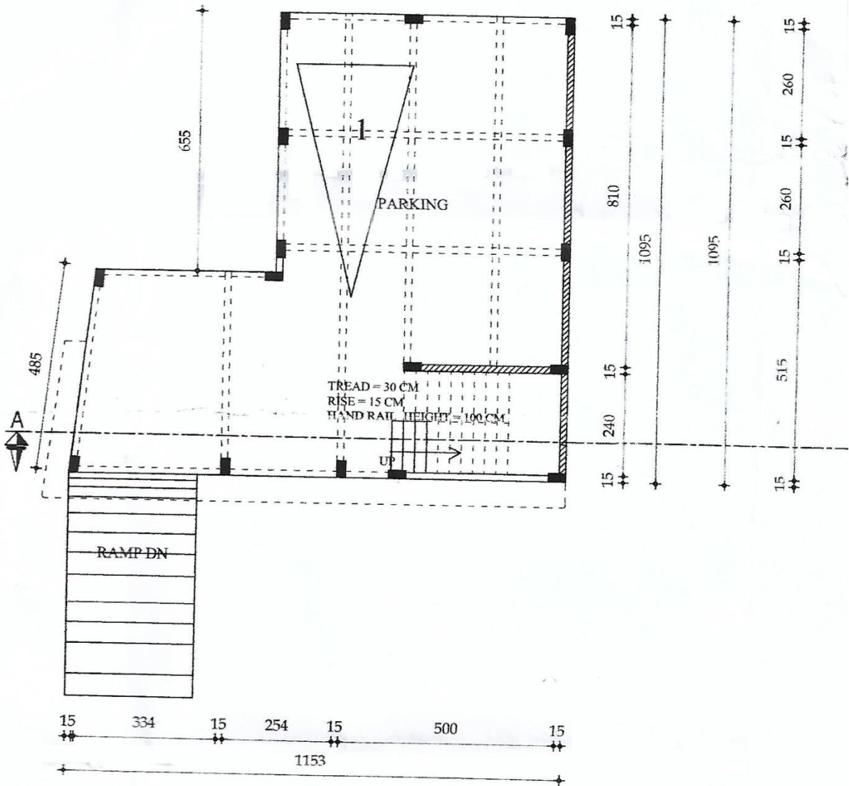
CELLAR FLOOR PLAN
